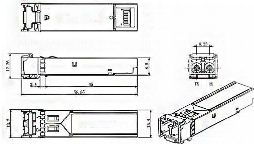
Figure 6. Mechanical Drawing
